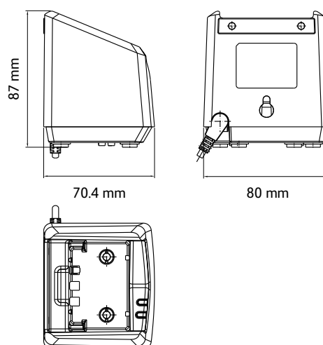
SAILOR CH 3505 Single Charger Unit
