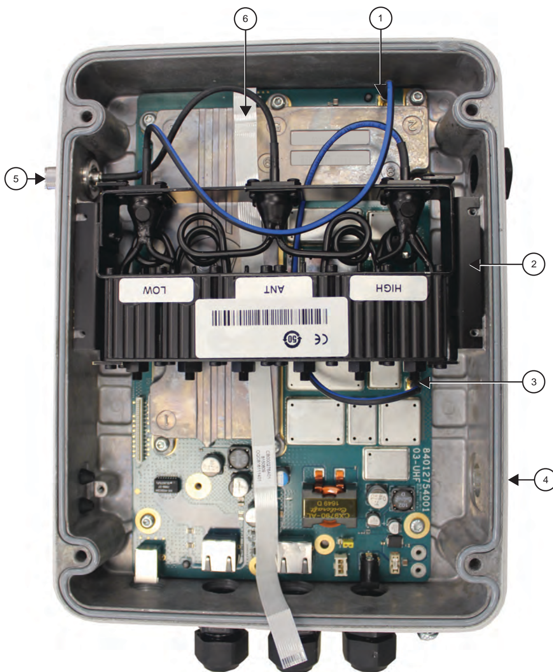
Figure 29: SLR 1000 Repeater Front View (without top cover) with a Duplexer
