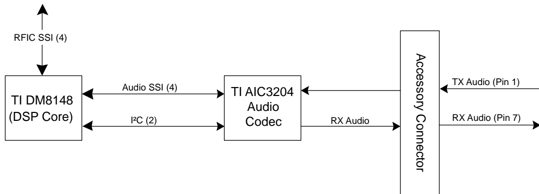
Figure 12: SLR 1000 Repeater Audio Block Diagram
