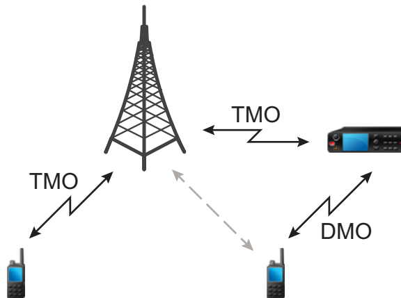
Figure 15: Gateway Mode Operation
