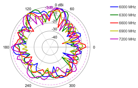
Elevation: 6000 – 7200 MHz
