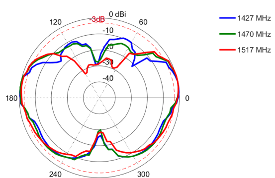
Elevation: 1427 – 1517 MHz
