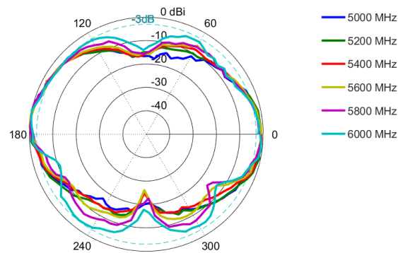
Elevation: 5000 – 6000 MHz
