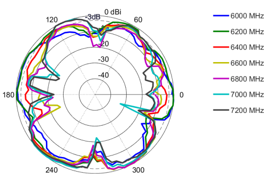
Elevation: 6000 – 7200 MHz
