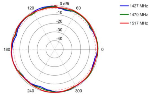
Azimuth: 1427 – 1517 MHz
