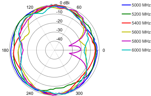
Azimuth: 5000 – 6000 MHz
