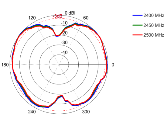
Elevation: 2400 – 2500 MHz
