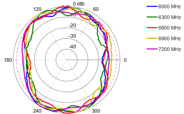
Azimuth: 6000 – 7200 MHz
