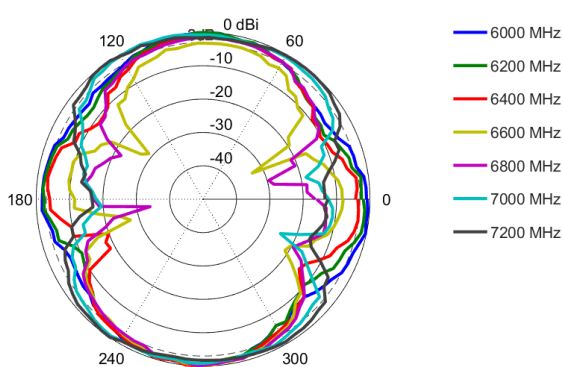
Azimuth: 6000 – 7200 MHz
